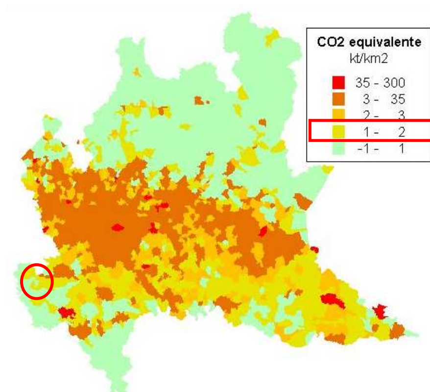
Figura 69: Gas serra (2010)
